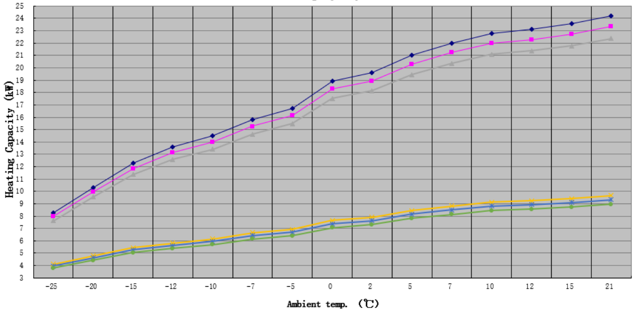
Curve of Heating Capacity Performance
